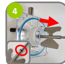
Remove Torque assembly and O-ring
