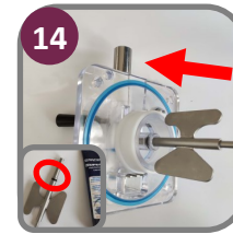
Install and Lubricate O-Ring; Install Torque Assembly
