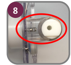
Rotate Draw Valve to Install Ice Buster
